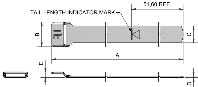
ONE STEP BAND STRAP - STRAIGHT
