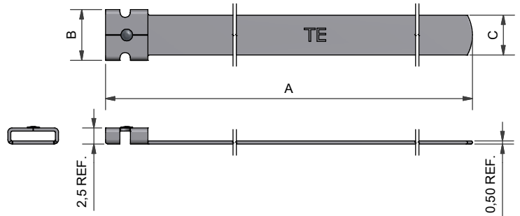
TWO STEP BAND STRAP - STRAIGHT
